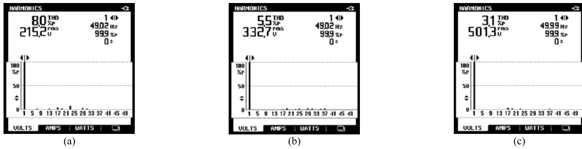
FIGURE 17. Harmonic spectrums of 11-level CHB MLI: (a) m = 0.3 , (b) m = 0.6 , (c) m = 1 .
