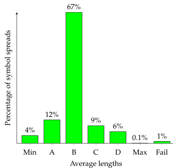
Figure 1. Distribution of average lengths of ANS encodings for the toy ANS. Note that H(\mathbb{S}) \approx 1.477 Legend: A = \langle Min, 1.48 \rangle , B = \langle 1.48, 1.49 \rangle , C = \langle 1.49, 1.5 \rangle , D = \langle 1.5, Max \rangle , Min = \frac{3619}{2448} \approx 1.478 and Max = \frac{97}{64} \approx 1.515 .
