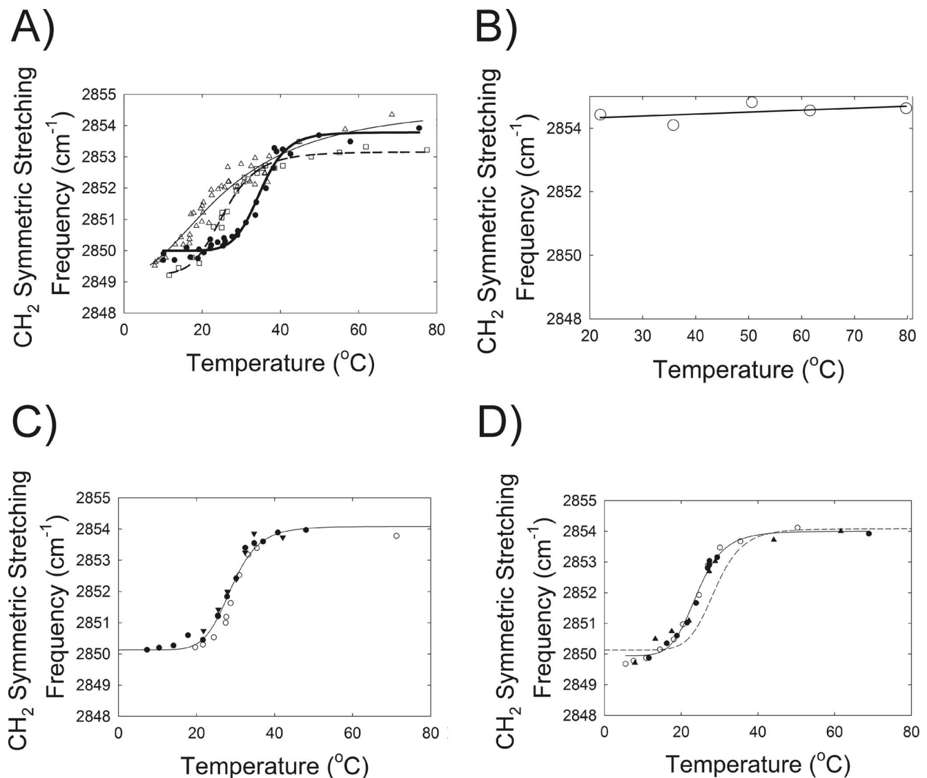
FIGURE 6. Order-disorder lipid phase transitions were measured using infrared spectroscopy. The infrared \text{CH}_2 symmetric stretching band center of mass (frequency) was measured to calculate trans/gauche rotamer ratios as a lipid order parameter. Higher center of mass values indicates more disorder in the hydrocarbon chains. (A) ( \Delta — \Delta ) Lipid phase transition of sebum from a 61-year-old Caucasian male. ( \square — \square ) Lipid phase transition of meibum from children mixed with sebum (20% by weight). ( \bullet — \bullet ) Lipid phase transition of meibum pooled from children. Phase transition parameters are provided in Table 2. (B) No order-disorder transition was detected for squalene through the temperature range measured. (C) Phase transitions for a pool of human meibum pooled from adults. (D) Phase transitions for a pool of human meibum pooled from adults and squalene (3:1, weight:weight). (—) Curve fit of data from Figure 3C for comparison. Phase transition parameters for the phase transitions are found in Table 3. (—) Curve fit to data. Symbols are separate experiments conducted on different days.
