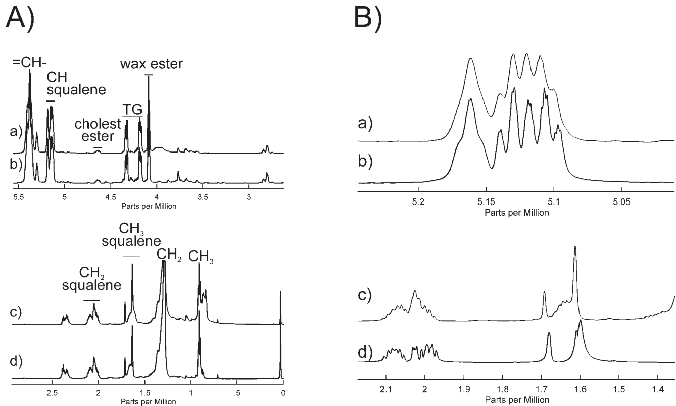
FIGURE 7. (A) ^1\text{H} NMR spectra of sebum from a 59-year-old Caucasian donor. The =\text{CH} resonance regions of (a) sebum extracted from tape (CuDerm Corp.); (b) sebum collected directly. The \text{CH}_2 and \text{CH}_3 resonance regions of (c) sebum extracted from tape (CuDerm Corp.); (d) sebum collected directly. (B) ^1\text{H} NMR spectra of: (a, c) sebum collected directly from a 59-year-old Caucasian donor; (b, d) squalene.
