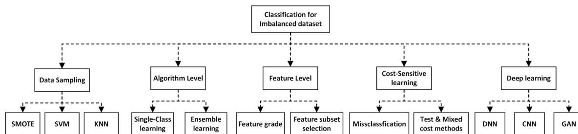
Fig. 5. The main techniques for classifying imbalanced datasets.
