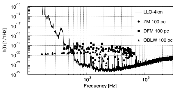
FIG. 13: Signal strength h_{\text{rss}} at the detectors versus central frequency for the 176 supernovae waveforms from the three models described in references [14, 15, 16]: the hydrodynamical model of ref. [14], labeled “ZM”, the relativistic effects considered in ref. [15] and labeled “DFM”, and finally the hydrodynamical model employing realistic nuclear equation of state of ref. [16], labeled “OBLW”. In all cases, the supernova events are positioned in optimal orientation and polarization at 100 pc from the detectors. The strain sensitivity of the L1 detector during the S2 run is shown for comparison.
