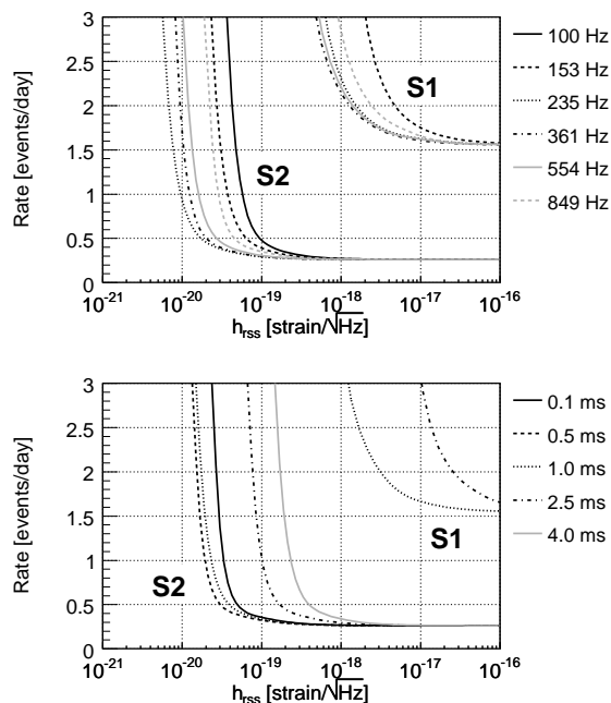
FIG. 12: Rate versus h_{TSS} exclusion plots at the 90% confidence level derived from the LIGO burst search using the S2 data. The top plot corresponds to burst events modeled by sine-Gaussians of Q=8.9 and frequencies ranging from 100 Hz to 849 Hz, while the bottom plot corresponds to ones events modeled by Gaussians of the \tau 's shown. For comparison, the corresponding curves resulting from the S1 analysis are superimposed.
