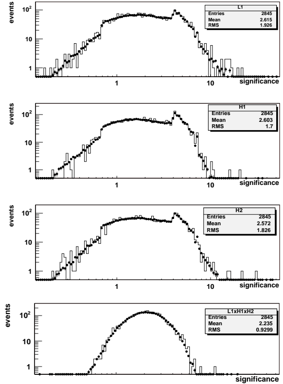
FIG. 3: The significance distribution of the triple coincident WaveBurst events for individual detectors (L1, H1, H2) and the combined significance of their triple coincidences (L1xH1xH2) for the S2 data set. Solid histograms reflect the zero-lag events, while the points represent background (time-lag) events as produced with unphysical time shifts between the Livingston and Hanford detectors (and normalized to the S2 live-time). The change in the significance distribution for the individual detectors around significance equal to four is attributed to the onset of single pixel clusters (for which a higher threshold was applied).
