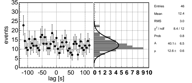
FIG. 5: WaveBurst event count (prior to the r -statistic test) versus lag time (in seconds) of the L1 interferometer with respect to H1 and H2. The zero-lag measurement, i.e. , the only coincidence measurement that is physical, is also shown. Due to the fragmentation of the data set, each time-lag has a slightly different live-time; for this reason, the event count is corrected so that they all correspond to the zero-lag live-time. A projection of the event counts to a one-dimensional histogram with a Poisson fit is also shown in the adjacent panel.
