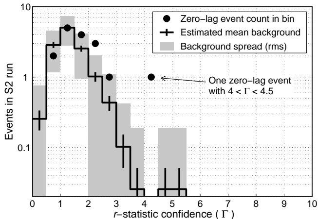
FIG. 6: Circles: histogram of r -statistic confidence value ( \Gamma ) for zero-lag events passing the WaveBurst analysis. Stair-step curve: mean background per bin, estimated from time lags, for an observation time equal to that of the zero-lag analysis. The black error bars indicate the statistical uncertainty on the mean background. The shaded bars represent the expected root-mean-square statistical fluctuations on the number of background events in each bin.
