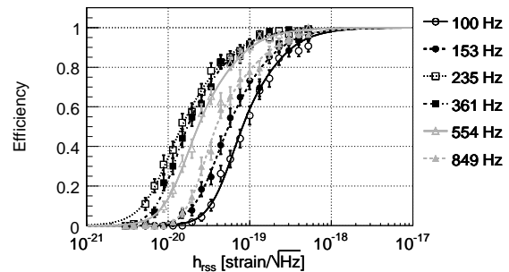
FIG. 8: Detection efficiency of the analysis pipeline as a function of the signal strength for sine-Gaussian waveforms of Q=8.9 and central frequencies of 100, 153, 235, 361, 554 and 849 Hz. The efficiencies plotted reflect averaging over random sky positions and polarization angles for injections covering the entire S2 data set. The x axis reflects the h_{\text{rss}} as defined in equation 8.2.
