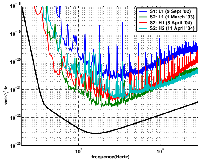
FIG. 1: Typical LIGO strain sensitivities in units of \text{Hz}^{-1/2} during the second science run (S2), compared to the most sensitive detector (L1) during the S1 science run. The solid line denotes the design goal for the 4 km instruments.
