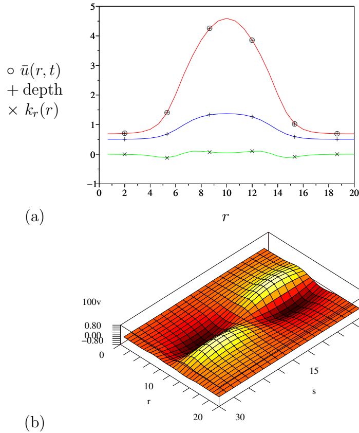
Figure 11: (a) an example channel is three times as deep in the middle as the surrounding shallows; the substrate has curvature k_r ; and the fluid flow is eight times as fast in the channel as in the shallows; (b) this base flow is unstable to superimposed travelling vortices on the shear near the sides of the channel as shown by the cross-channel velocity. Here \text{Re} = \text{Gr} = 80 on a substrate at angle \vartheta = 0.1 rad, with \text{We} = 0 .
