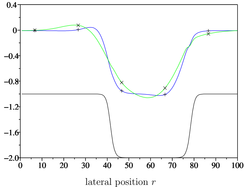
Figure 12: fluid film thickness for two Weber numbers We = 10 (+) and 100 ( \times ) for flow to the right over the shown substrate with a smoothed step-down and a smoothed step-up, as predicted by model (79–81): for near Stokes flow, Re = 0.1 ; scaled to the gravitational forcing Gr = 1 ; on a substrate at an angle \theta = 0.2 rad to the horizontal.
