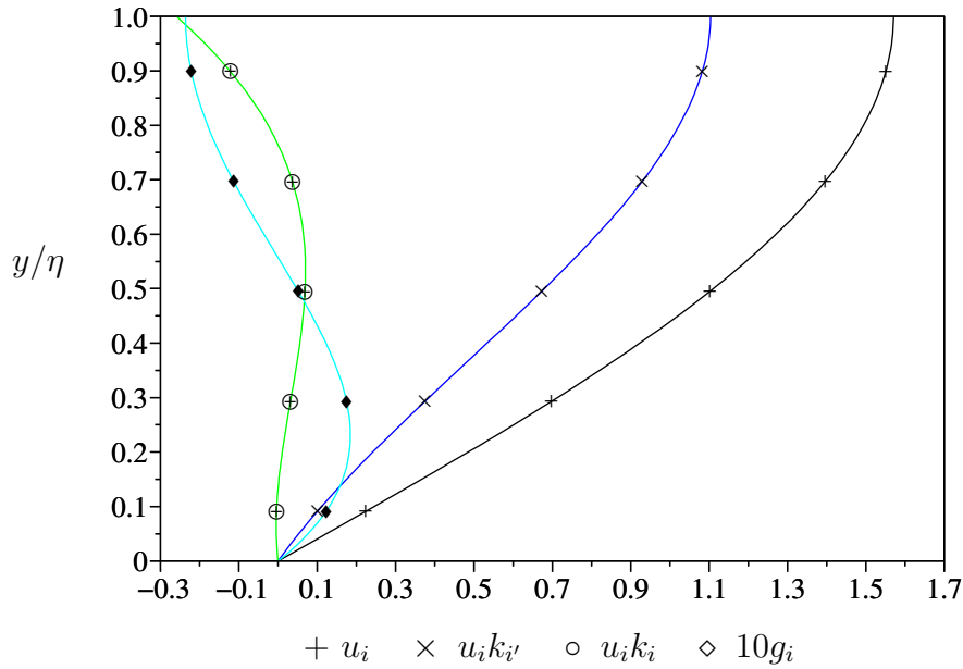
Figure 4: the normal structure of the lateral velocity field (51): +, component \propto \bar{\mathbf{u}} ; \times , component \propto k_{i'} u_i ; \circ , component \propto k_i u_i ; and \diamond , 10 \times component \propto \text{We} \nabla \kappa + \text{Gr} \mathbf{g}_s .
