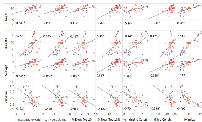
Figure 3: Scatter plot and correlation of diversification indicators and research performance indicators.
