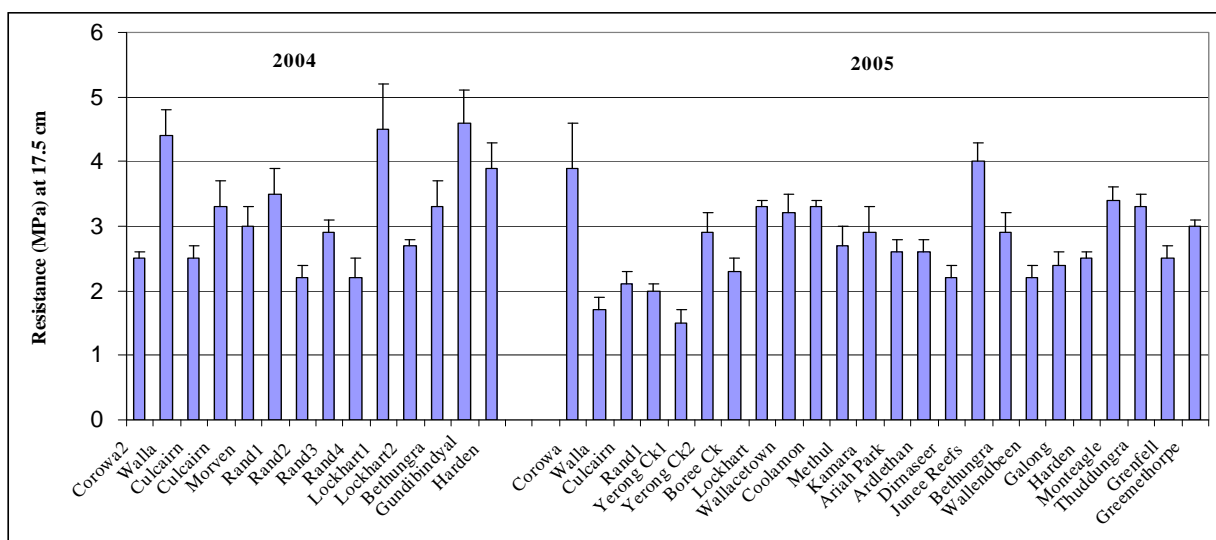
Figure 1. Penetrometer resistance (MPa) measured below the disturbed surface layer (17.5 cm depth) in winter for paddocks across southern NSW in 2004 and 2005.
